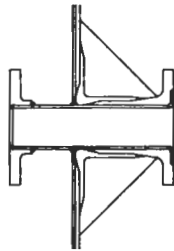
Formed Face Mounting Pad With Flanged Nozzle
